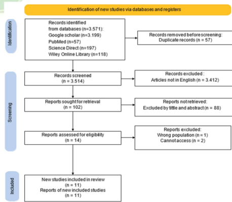
Figure 1. PRISMA Flowchart
