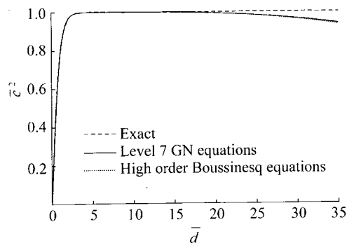
Fig.2 Comparison of dispersion relationships between Level 7 GN equations and high order Boussinesq equations (Madsen et al., 2006)
