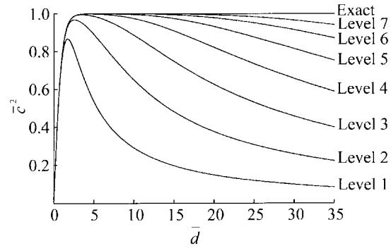
Fig.1 Dispersion relationships of the GN equations
